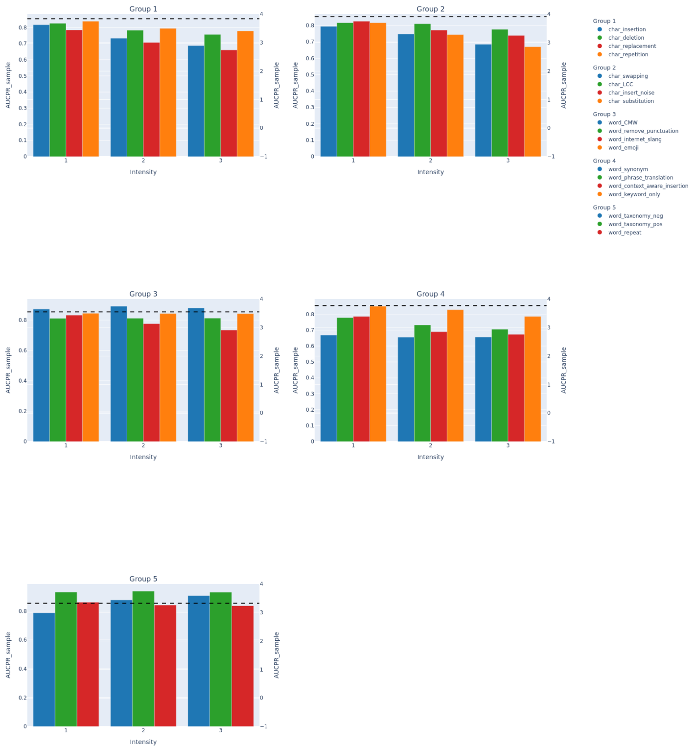
Grouped Bar Plots of AUCPR_sample by Perturbation Type and Intensity
