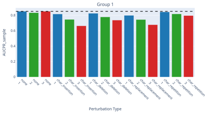
Highlighted Grouped Bar Plots of AUCPR_sample by Perturbation Type and Intensity
