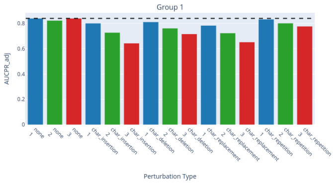
Highlighted Grouped Bar Plots of AUCPR_adj by Perturbation Type and Intensity
