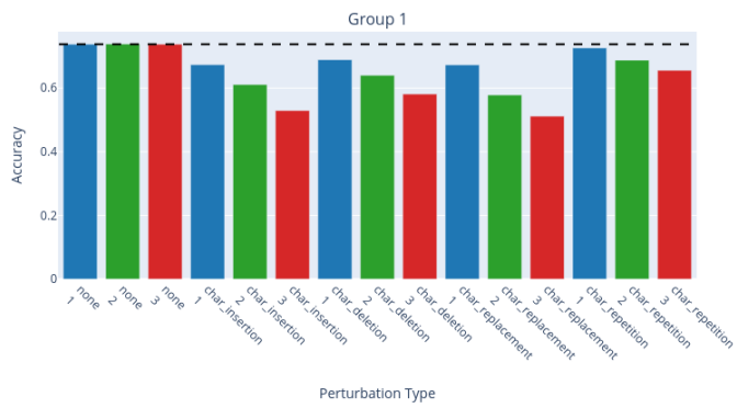
Highlighted Grouped Bar Plots of Accuracy by Perturbation Type and Intensity
