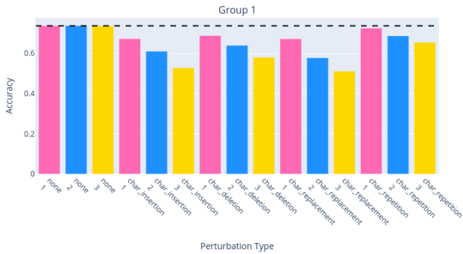
Grouped Bar Plots of Accuracy by Perturbation Type and Intensity
