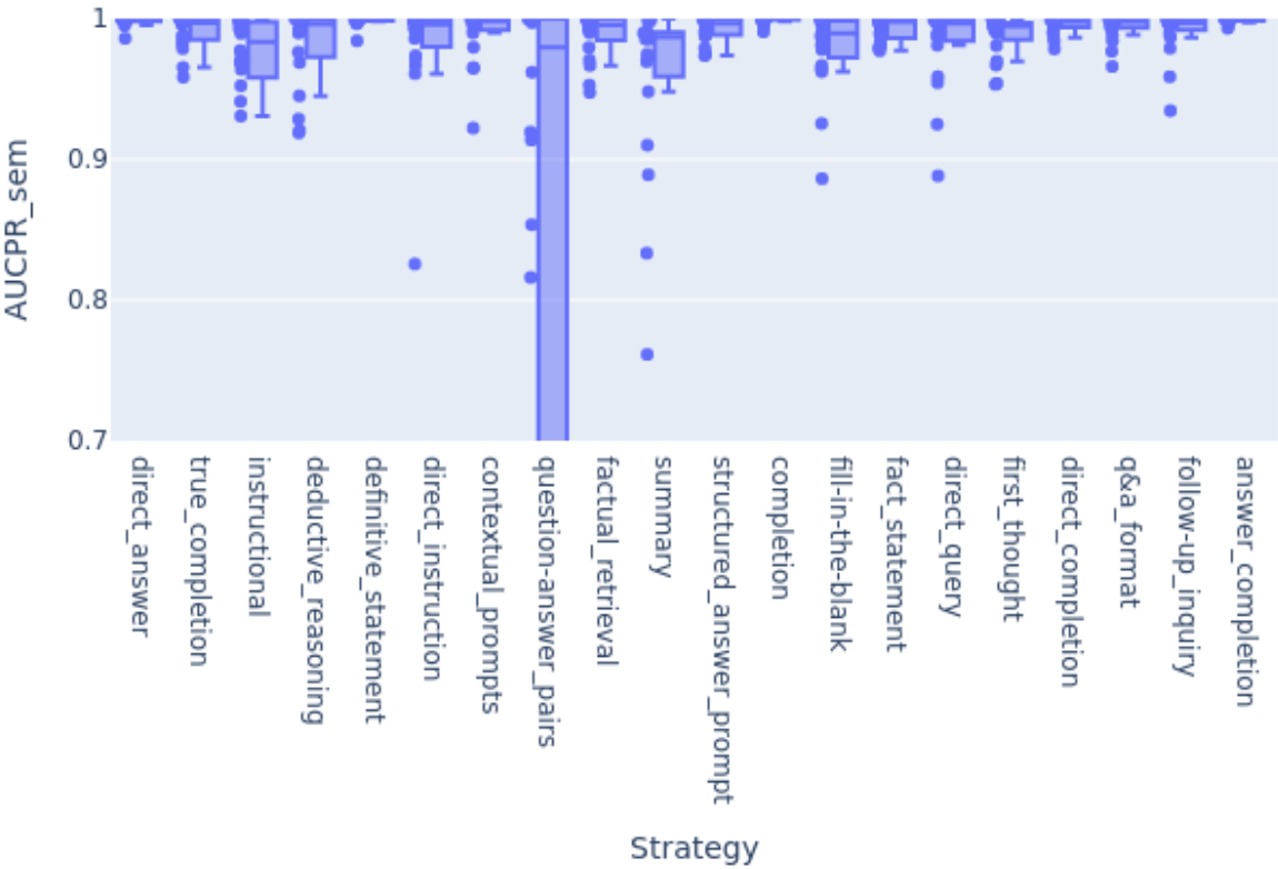
AUCPR_sem by Strategy and Dataset (Restricted Y-axis)
