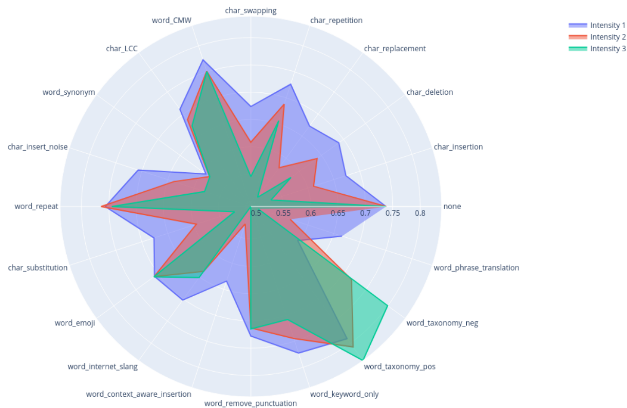
Radar Plot of Accuracy for Different Typo Types and Intensities
