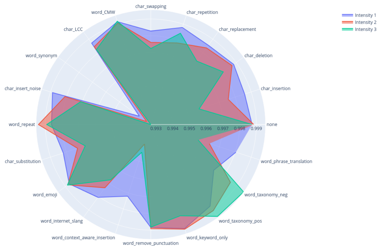
Radar Plot of AUCPR_sem for Different Typo Types and Intensities
