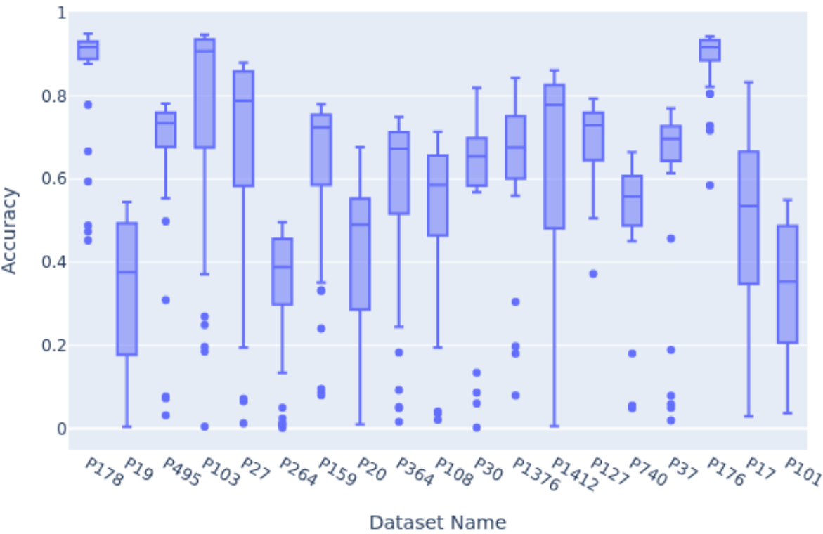
Accuracy by Dataset (Taxonomy Type: 0)
