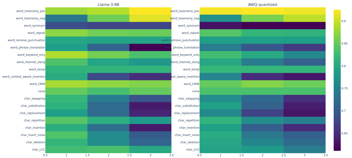
Heatmap of AUCPR_adj for Different Perturbation Types and Intensities
