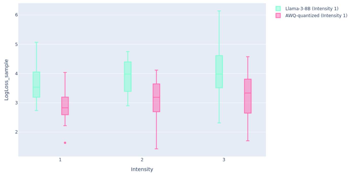
Distribution of LogLoss_sample across Intensities
