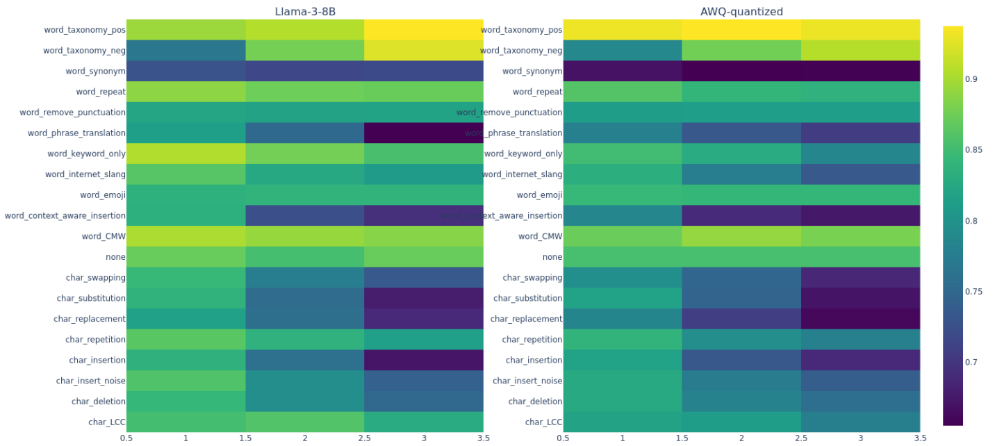
Heatmap of AUCPR_sample for Different Perturbation Types and Intensities
