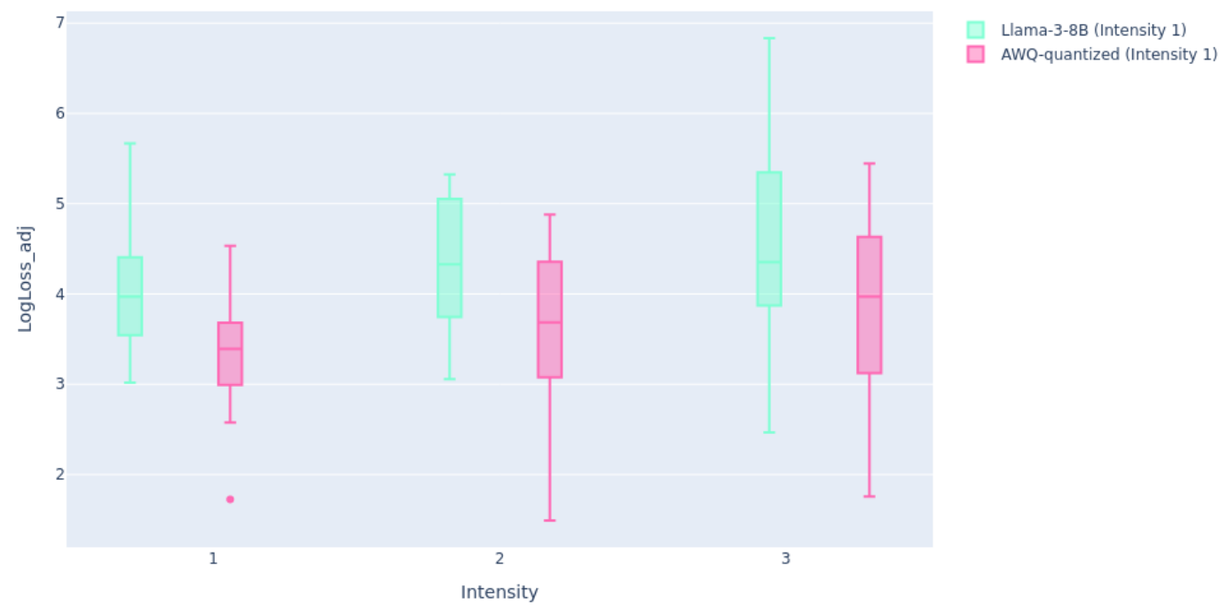
Distribution of LogLoss_adj across Intensities
