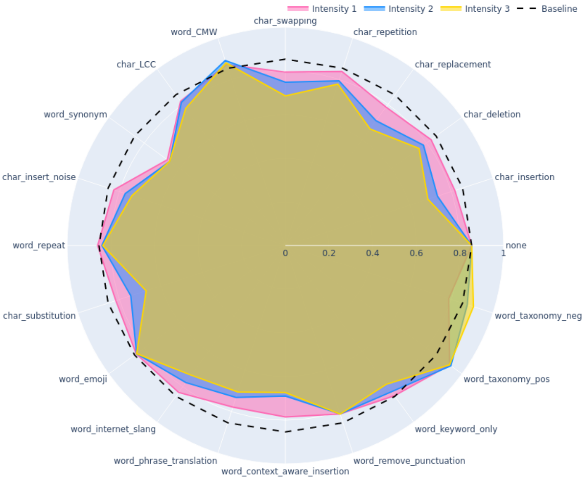
Radar Plot of AUCPR_sample
