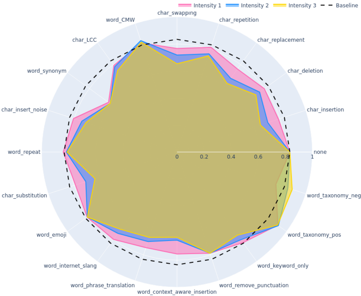
Radar Plot of AUCPR_adj
