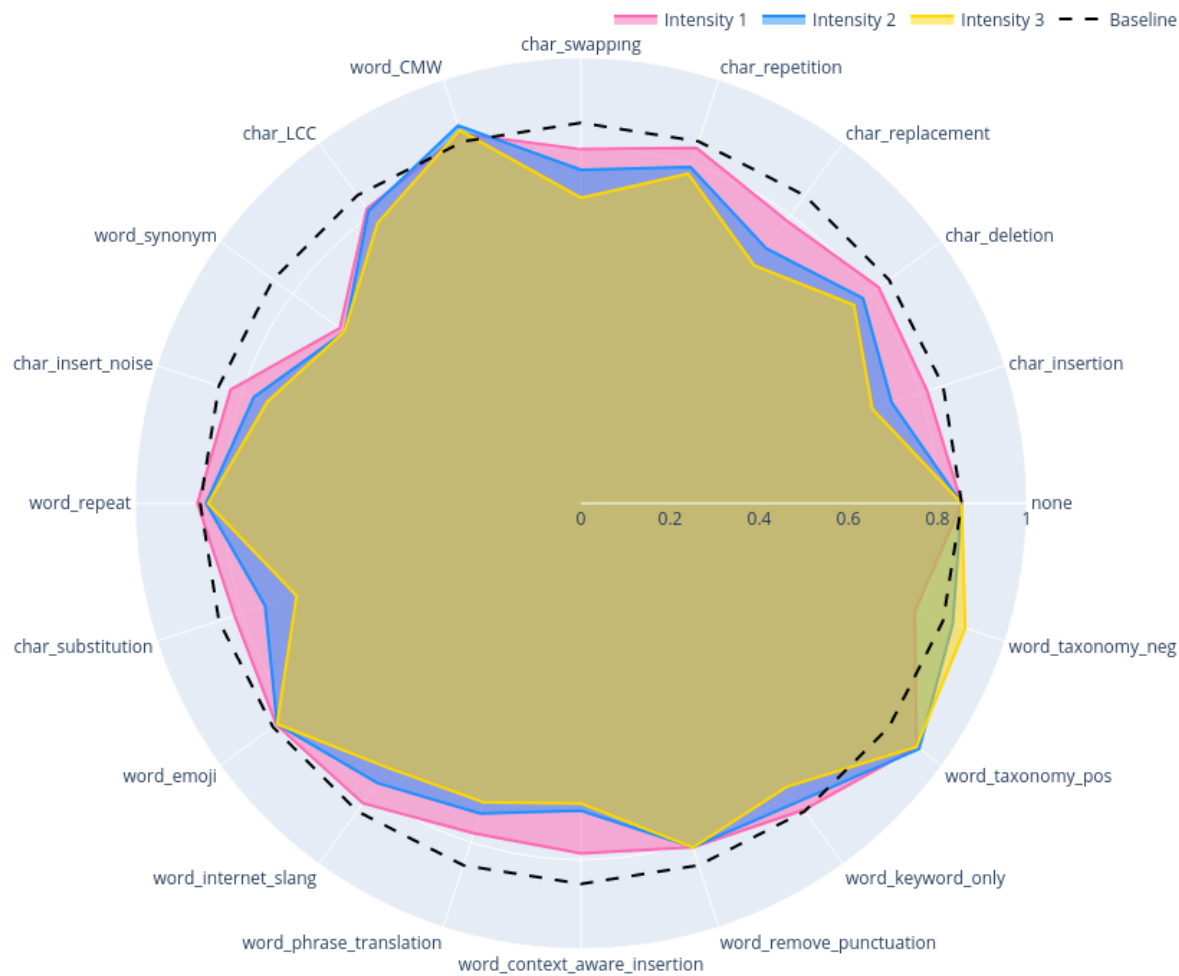
Radar Plot of AUCPR_sample
