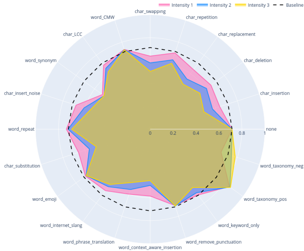
Radar Plot of Accuracy
