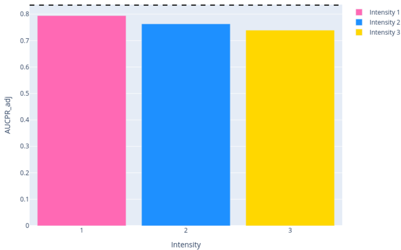
Aggregated Bar Plot of AUCPR_adj by Intensity
