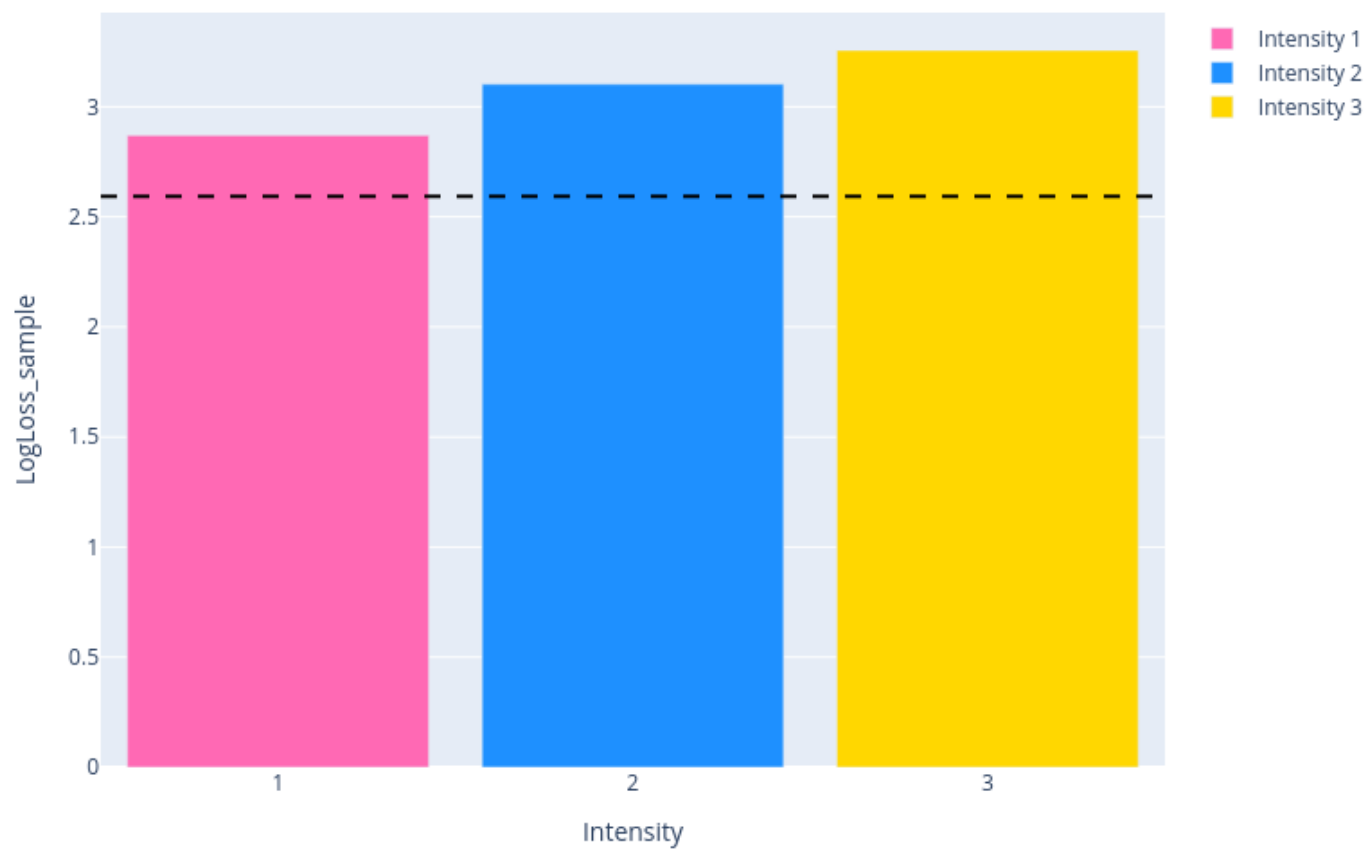
Aggregated Bar Plot of LogLoss_sample by Intensity
