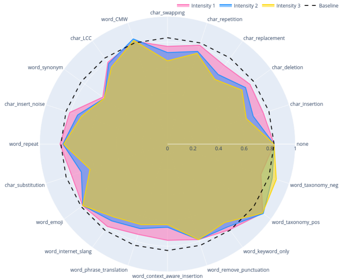
Radar Plot of AUCPR_adj
