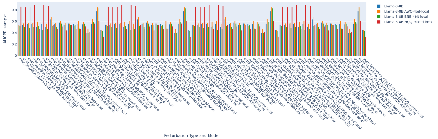
Model Comparison Bar Plot of AUCPR_sample for Intensity 1
