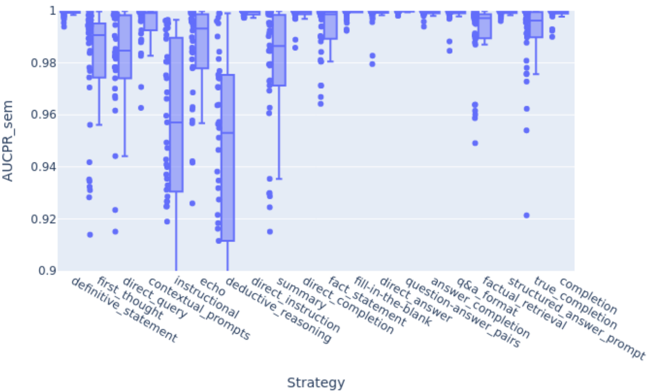
AUCPR_sem by Strategy and Dataset (0.9 to 1.0) (Taxonomy Type: 0)
