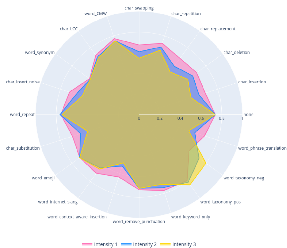
Radar Plot of Accuracy
