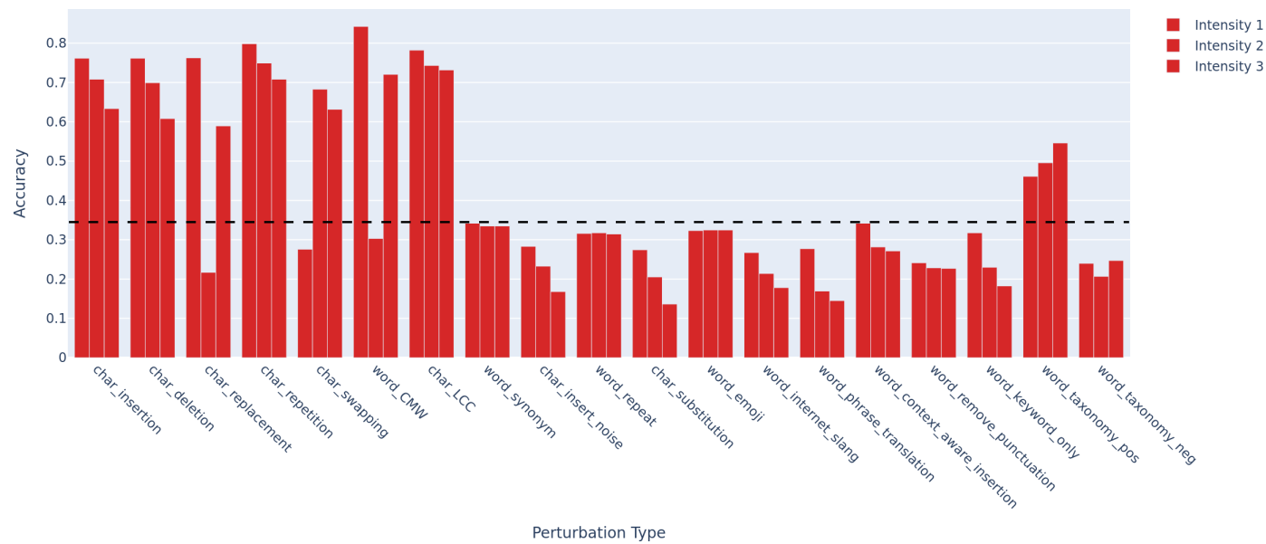
All Perturbations Bar Plot of Accuracy for Llama-3-8B-HQQ-mixed-local
