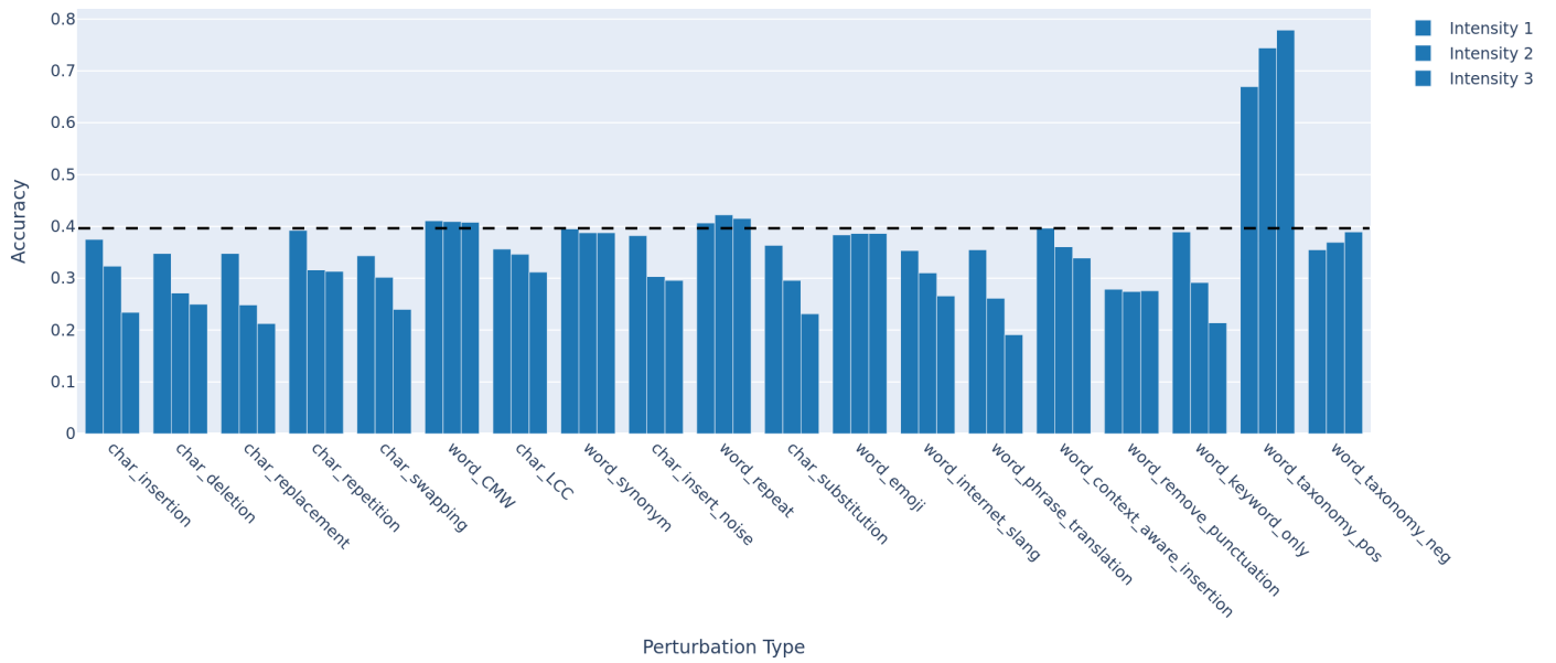
All Perturbations Bar Plot of Accuracy for Llama-3-8B
