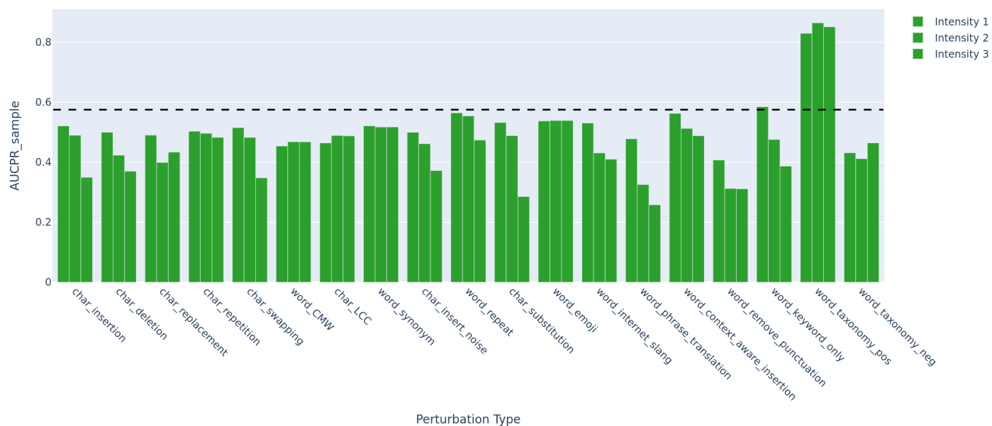
All Perturbations Bar Plot of AUCPR_sample for Llama-3-8B-BNB-4bit-local
