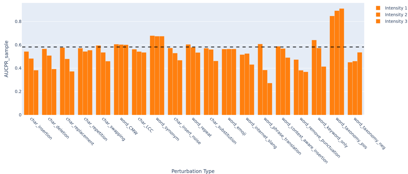
All Perturbations Bar Plot of AUCPR_sample for Llama-3-8B-AWQ-4bit-local
