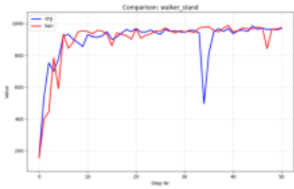
Comparison_walker_stand.png
