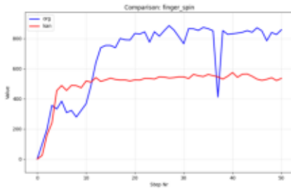
Comparison_finger_spin.png
