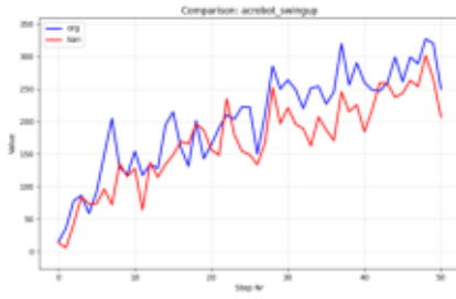
Comparison_acrobot_swingup.png
