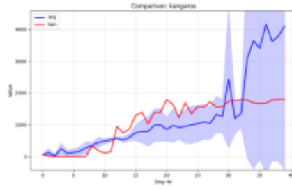
Comparison_kangaroo.png
