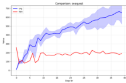
Comparison_seaquest.png
