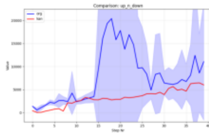
Comparison_up_n_down.png
