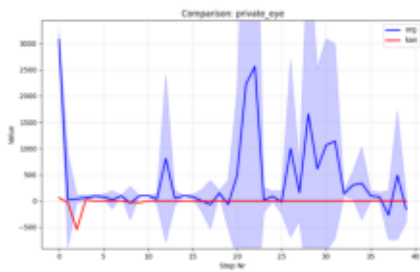
Comparison_private_eye.png
