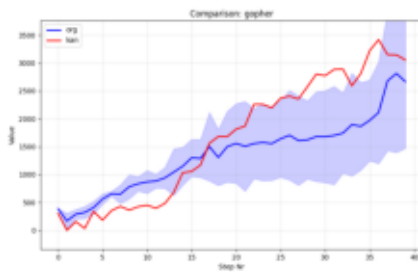
Comparison_gopher.png
