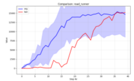
Comparison_road_runner.png
