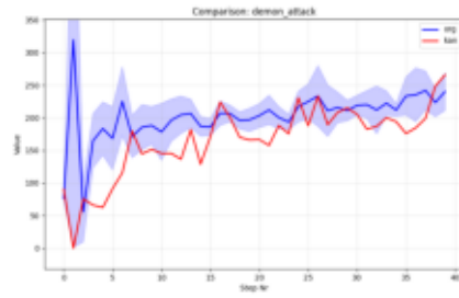
Comparison_demon_attack.png
