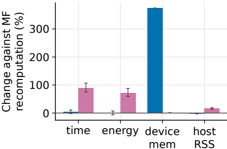
(a) MNIST 2×1000
