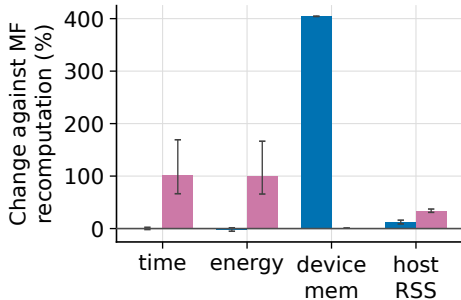
(b) Fashion-MNIST 2×1000
