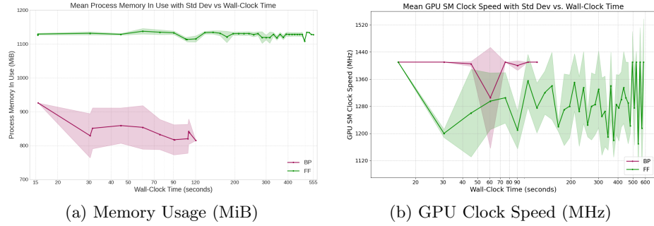
Fig. 2. Hardware-level autopsy of FF vs. BP on the Fashion-MNIST 4 \times 2000 MLP. FF consumes slightly more peak GPU memory than BP, contradicting the theoretical expectation that eliminating the backward pass reduces memory. FF also exhibits volatile GPU clock speeds indicating underutilisation of the compute pipeline, whereas BP maintains stable, high clock rates. Trace labels follow the WiMj convention: W_i = weight matrix i , M_j = monitor channel j . Dataset: Fashion-MNIST; Architecture: 4 \times 2000 MLP.
