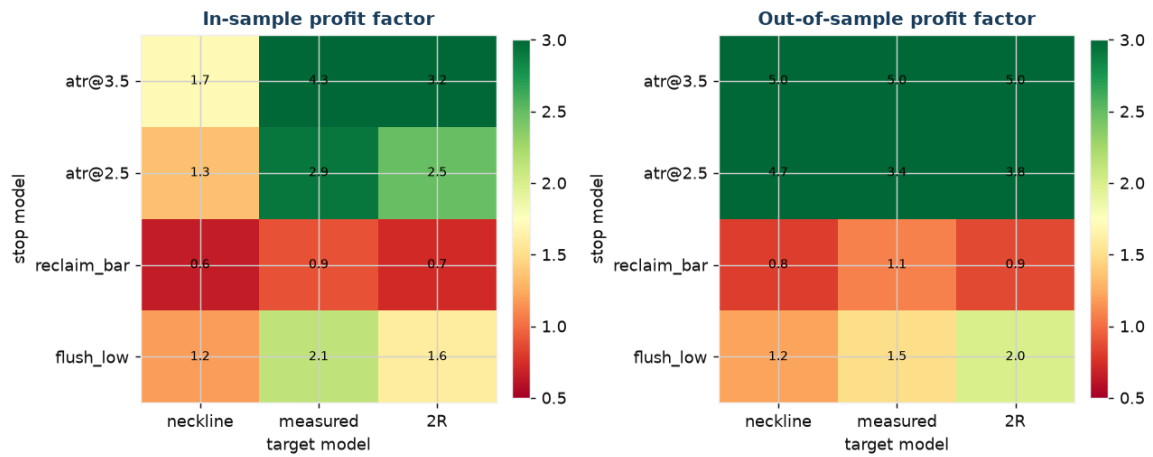
Figure 5. Profit factor for every stop-model (rows) x target-model (columns) combination, in-sample (left) vs out-of-sample (right); greener is better. The ATR-stop rows stay green in both panels; the tight reclaim-bar stop is red; the original flush-low/neckline corner fades. Only settings green in BOTH panels are trustworthy.
