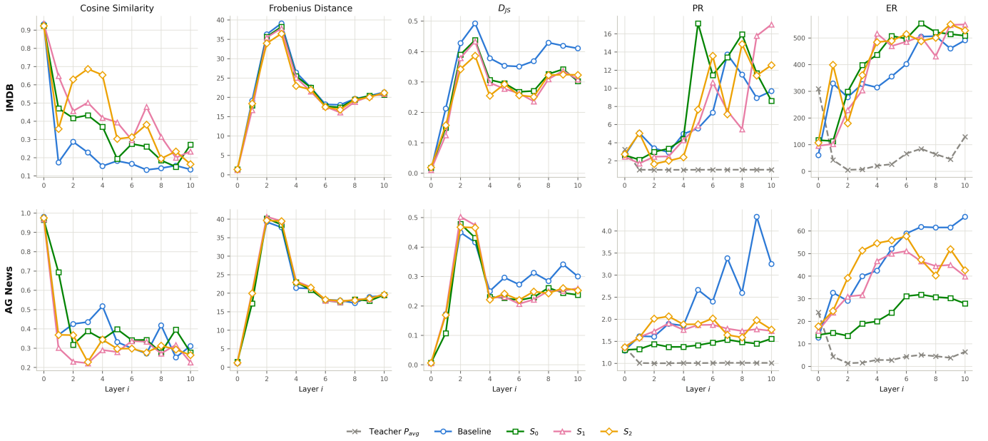
Figure 1: Cosine similarity, Frobenius distance, row-averaged Jensen–Shannon divergence ( D_{JS} ), Participation Ratio (PR), and Entropy Rank (ER) between each model’s attention maps and the teacher’s P_{avg} , both averaged over the test set (following P_{avg_i} = (P_{2i} + P_{2i+1})/2 for layer i from teacher model P ), for the non-distilled baseline ( B ) and the distilled students ( S_0 , S_1 , S_2 ), on both datasets IMDb and AG News .
