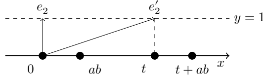
Figure 2.5: Translating [0, ab] by t in \mathbb{R}^1 .
