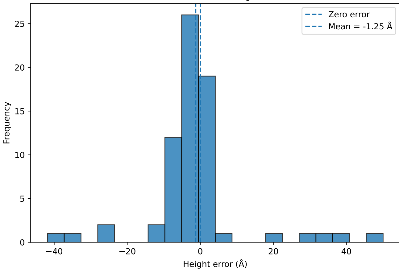
Distribution of QD Height Errors
