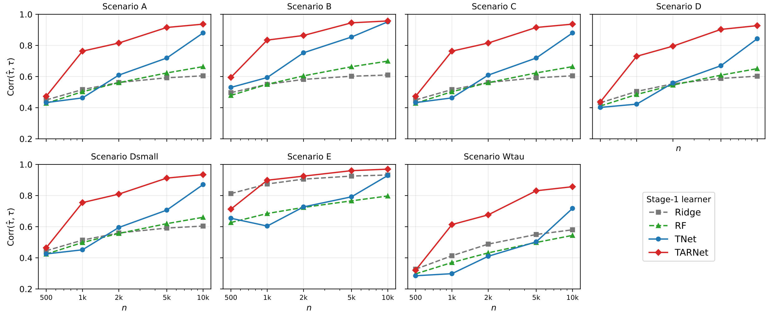
Stage-1 CATE quality: correlation vs n (higher is better)
