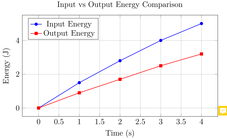
Figure 3: Input and output energy comparison. Losses are due to internal resistance, parasitic capacitance, and electromechanical coupling efficiency.
