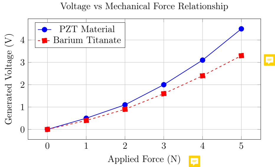
Figure 1: Generated voltage versus applied force. PZT shows higher sensitivity and efficiency at low forces, indicating its advantage in micro-vibration harvesting.
