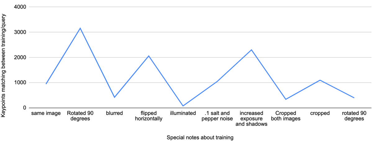
Keypoints matching between training/query vs. Special notes about training
