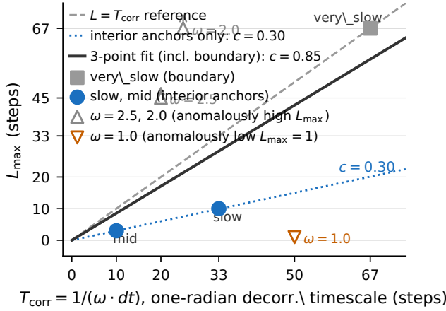
Figure 1: L_{\max} (last significant L , window method) vs. T_{\text{corr}} = 1/(\omega \cdot dt) . Filled circles: two clean interior anchors (slow, mid) on the c=0.30 line; open square: very_slow (boundary, consistent with c=0.30 but censored); open upward triangles: \omega=2.5 and \omega=2.0 (anomalously high L_{\max} , excluded from fit); open downward triangle: \omega=1.0 (anomalously low L_{\max}=1 , excluded from fit). Dashed: L=T_{\text{corr}} reference; solid: force-through-origin fit on two interior anchors plus boundary point ( c=0.85 , inflated by censoring); dotted: c=0.30 through the two interior anchors.
