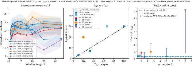
Figure 4: Reward-optimal window sweep ( n=16 seeds, shared arm only, exploratory). L_{\text{opt}}(\omega) denotes the L maximising shared-arm reward — distinct from L_{\text{max}} (last significant \bar{\Delta} ) and from L^* (zero-crossing of \mathbb{E}[\bar{\Delta}] ). Left: Shared-arm reward vs. L for \omega \in \{0.5, 0.75, 1.0, 1.5, 2.5, 5.0, 8.0\} . Linear-regime curves (solid blue) have reward peaks at moderate L ; anomalous conditions (dashed) are flat or boundary-limited. Centre: L_{\text{opt}}(\omega) vs. T_{\text{corr}} = 1/(\omega \cdot dt) . Filled circles: three linear-regime points; dashed line: force-through-origin fit, slope 0.29. Open markers: anomalous-regime points, excluded from fit. Right: \Gamma(\omega) = \omega \cdot dt \cdot L_{\text{opt}} vs. \omega with bootstrap 95% CIs ( B=4000 seed resamples). The \pm 20\% band is shown for reference; the \omega=1.5 point lies below it, and all three linear-regime CIs are wide, reflecting argmax instability with n=16 seeds over ten discrete L values. The result is suggestive but not confirmatory.
