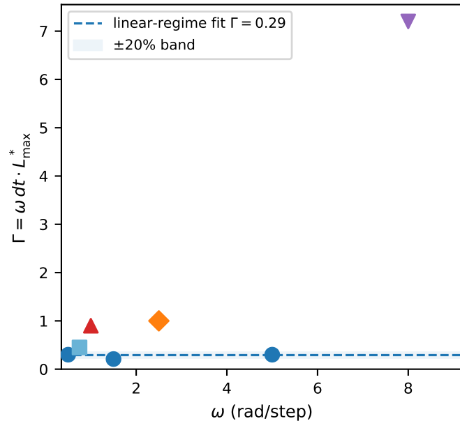
Dimensionless group \Gamma(\omega)
