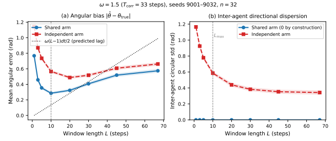
Figure 3: Directional diagnostics, \omega=1.5 (slow, n=32 seeds, 9001–9032). Shaded bands are \pm 1 SE across seeds. (a) Mean angular error |\hat{\theta} - \theta_{\text{true}}| vs. L . Shared arm (blue) shows an observed minimum at L=10 (0.286 rad), then rises as predicted angular lag \omega(L-1)dt/2 (dotted) accumulates. Adjacent-comparison tests support the minimum ( E_{\text{shared}}(5) > E_{\text{shared}}(10) : t=3.76 ; E_{\text{shared}}(20) > E_{\text{shared}}(10) : t=1.89 ; both unpaired). Independent arm (red) decreases monotonically. (b) Inter-agent directional dispersion (circular std across agents). Shared arm is identically zero for all L by construction; independent arm retains 0.585 rad at L=10 , 0.343 rad at L=67 . Zero shared-arm dispersion is structural, not a collapse at L_{\text{max}} ; the harmful regime is zero diversity combined with a stale direction.
