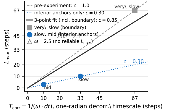
Figure 1: L_{\text{max}} (last significant L , window method) vs. T_{\text{corr}} = 1/(\omega \cdot dt) . Filled circles: two clean interior anchors (slow, mid); square: very_slow (boundary); triangle: \omega=2.5 (shown for reference — no reliable L_{\text{max}} , excluded from fit). Dashed: pre-experiment prediction ( c=1.0 ); solid: force-through-origin fit on three reliable points including boundary very_slow ( c=0.85 , inflated by boundary censoring); the two interior anchors alone give c=0.30 exactly. fast ( T_{\text{corr}}=3 ) has no reliable L_{\text{max}} and is omitted.
