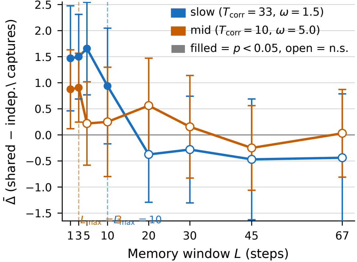
Fig. 2. \bar{\Delta} (mean shared – independent captures, \pm 95\% CI) vs. memory window L for slow ( T_{\text{corr}}=33 , blue) and mid ( T_{\text{corr}}=10 , orange), window method, n=32 seeds. Filled markers: p < 0.05 ; open markers: not significant. Dashed verticals mark L_{\text{max}} for each speed. The crossover for slow is sharp: +0.94 at L=10 to -0.38 at L=20 , a swing of >1.3 particles.
