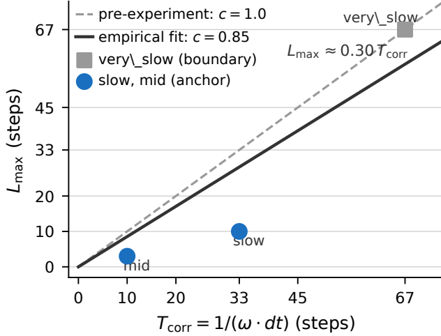
Figure 1: L_{\text{max}} (last significant L , window method) vs. T_{\text{corr}} = 1/(\omega \cdot dt) . Filled circles: two clean interior points (slow, mid); square: very_slow (boundary — any L_{\text{max}} \in [45, 67] maps to 67 in our L grid). Dashed: pre-experiment prediction ( c=1.0 ); solid: force-through-origin fit on three points including the boundary very_slow ( c=0.85 , inflated by boundary censoring); the two interior anchors alone give c=0.30 exactly. fast ( T_{\text{corr}}=3 ) has no reliable L_{\text{max}} and is omitted.
