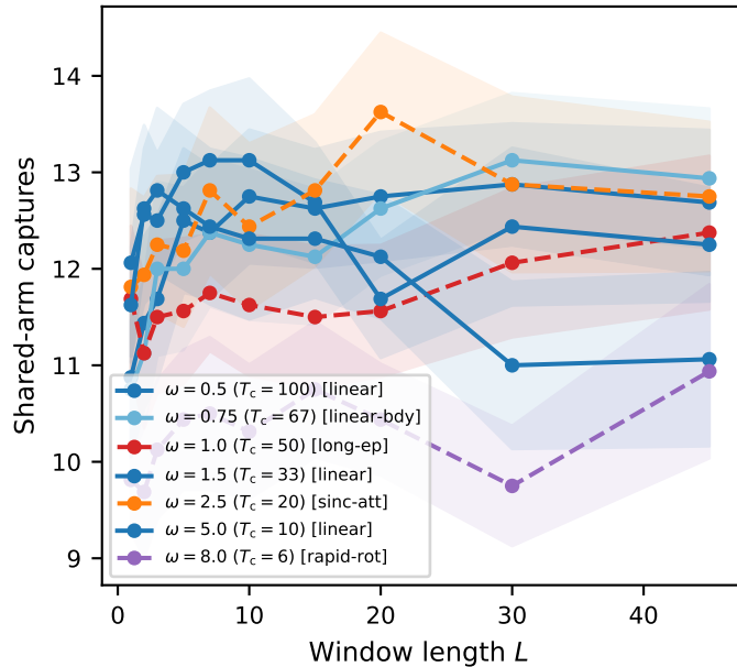
Shared-arm reward vs. L
