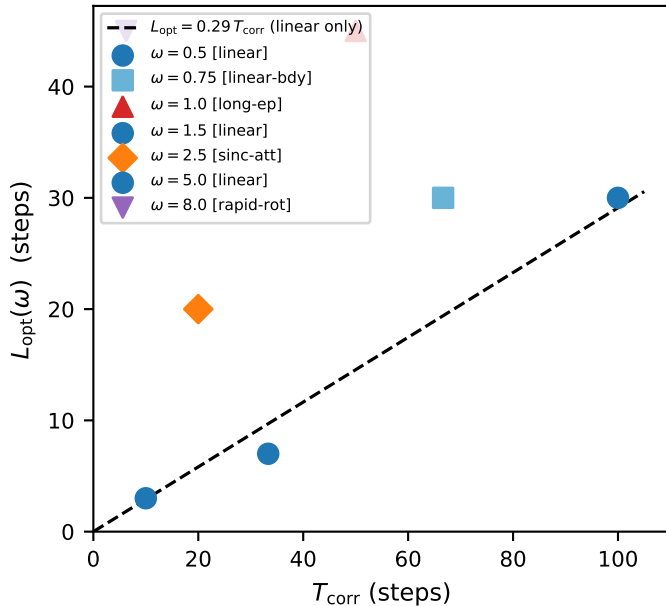
L_{\text{opt}} vs. T_{\text{corr}}
