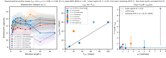
Figure 4: Reward-optimal window sweep ( n=16 seeds, shared arm only, exploratory). L_{\text{opt}}(\omega) denotes the L maximising shared-arm reward — distinct from L_{\text{max}} (last significant \Delta ) and from L^* (zero-crossing of \mathbb{E}[\Delta] ). Left: Shared-arm reward vs. L for \omega \in \{0.5, 0.75, 1.0, 1.5, 2.5, 5.0, 8.0\} . Linear-regime curves (solid blue) have reward peaks at moderate L ; anomalous conditions (dashed) are flat or boundary-limited. Centre: L_{\text{opt}}(\omega) vs. T_{\text{corr}} = 1/(\omega \cdot dt) . Filled circles: three linear-regime points; dashed line: force-through-origin fit, slope 0.29. Open markers: anomalous-regime points, excluded from fit. Right: \Gamma(\omega) = \omega \cdot dt \cdot L_{\text{opt}} vs. \omega with bootstrap 95% CIs ( B=4000 seed resamples). The \pm 20\% band is shown for reference; the \omega=1.5 point lies below it, and all three linear-regime CIs are wide, reflecting argmax instability with n=16 seeds over ten discrete L values. The result is suggestive but not confirmatory.
