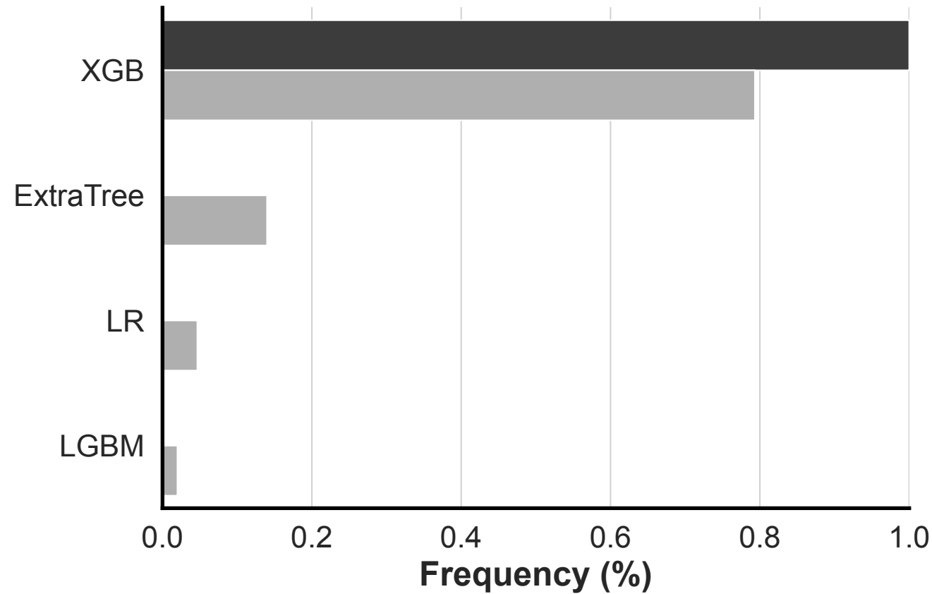
adult
