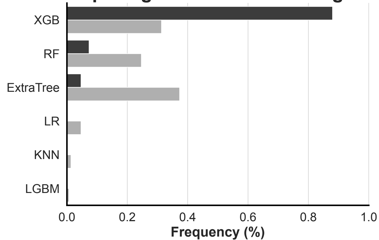
portuguese-bank-marketing
