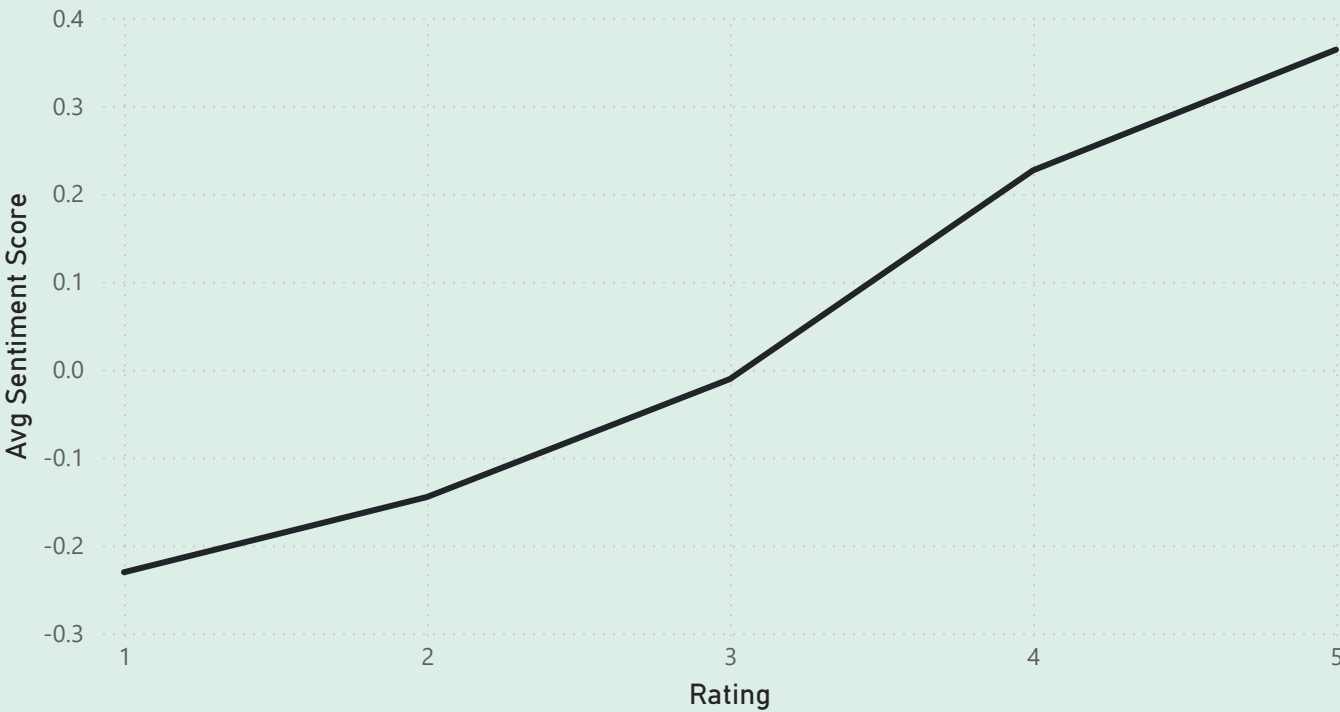
Avg Sentiment Score by Rating
