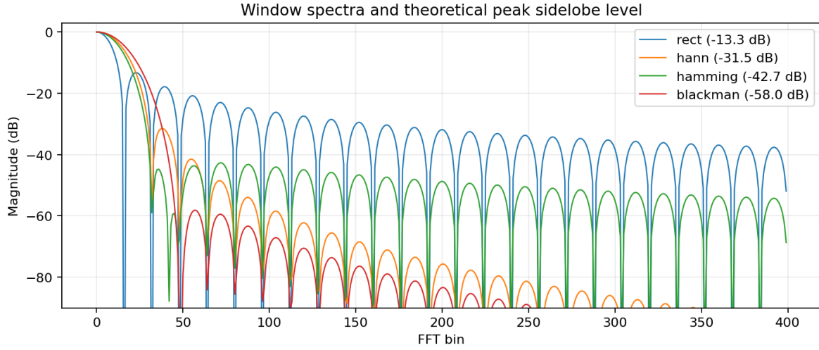
Fig. 7. Envelope windows and their sidelobe floors. Selection is by predicted margin: Hann below 3 dB, Blackman above 400 NTU, Hamming otherwise.
