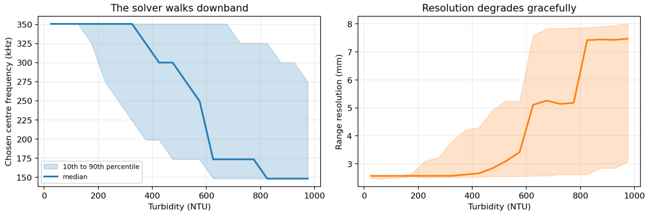
Fig. 13. Selected centre frequency and the resulting range resolution against sediment load, over 20,000 decisions. The band is the 10th to 90th percentile. Resolution degrades gracefully rather than the return being lost.
