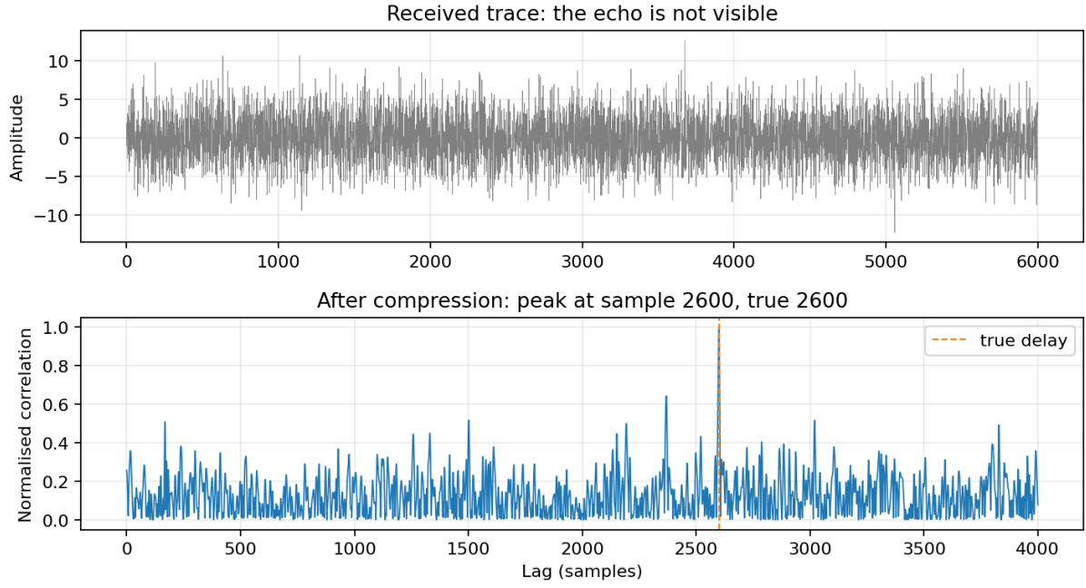
Fig. 9. Matched filtering. Upper: the received trace, in which the echo is not visible. Lower: the correlator output, with the peak at the true delay marked.
