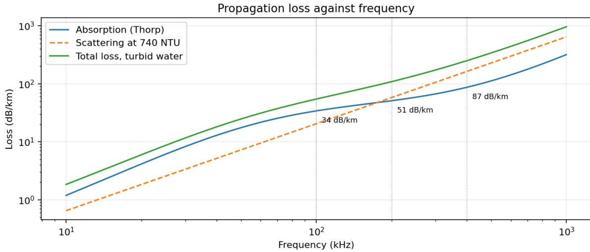
Fig. 2. Propagation loss against frequency. Absorption follows Thorp's expression; the dashed trace is the scattering contribution at 740 NTU; the upper trace is their sum. The vertical markers are 100, 200 and 400 kHz. Computed by thorpDbPerKm() in src/core/physics.ts .
