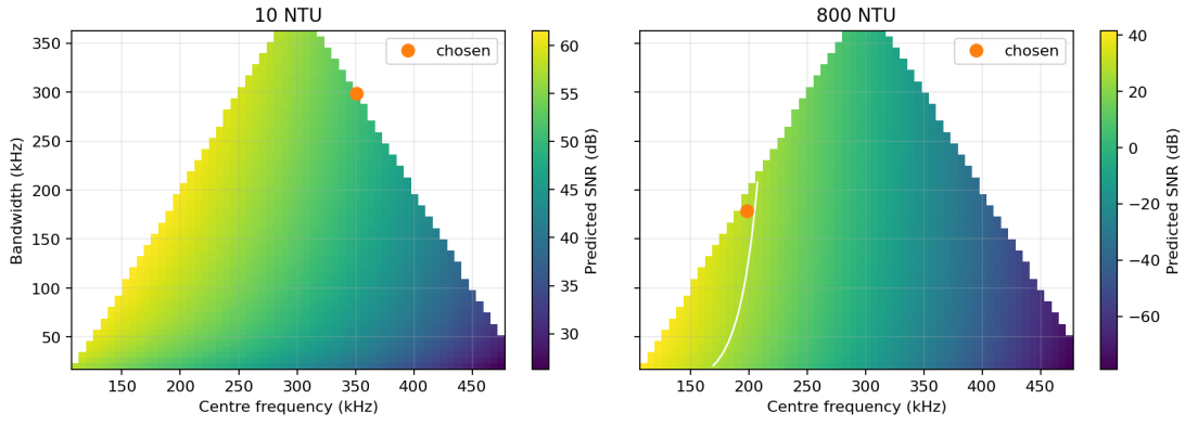
Fig. 12. Predicted signal-to-noise ratio across the candidate grid in clear and in turbid water. The contour marks the detection threshold plus margin. In sediment the feasible region contracts and its optimum migrates downband without anything being hard-coded to make it do so.
