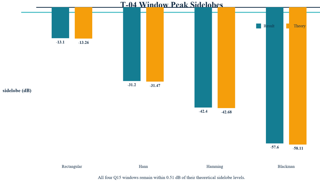
Fig. 8. Measured sidelobe structure for the four windows T-04 . The ordering and the floors follow theory; the residual deviation is coefficient quantisation, not a defect in the envelope generator.
