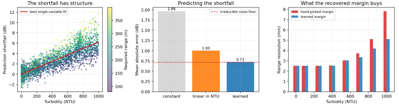
Fig. 18. Left: the prediction shortfall against turbidity, coloured by required range; the spread resolves into structure once the second variable is conditioned on. Centre: accuracy against two baselines and the noise floor. Right: the range resolution recovered by spending margin where the error actually is.
