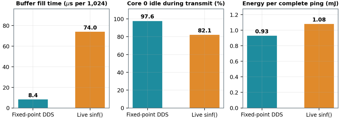
Fig. 16. Synthesis cost T-12 . Fixed-point direct digital synthesis fills 1,024 samples in 8.4\mu\text{s} against 74.0\mu\text{s} for live trigonometry, an 8.8 \times reduction that carries a 13.9% reduction in ping energy.
