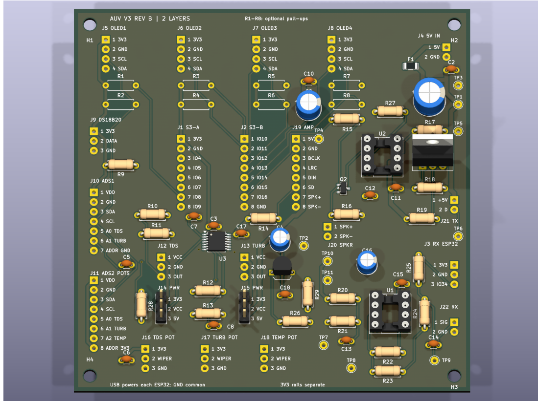
Fig. 1. Revision-B PCB layout and connector arrangement from the project KiCad files. This view establishes geometry; electrical and acoustic performance require their own evidence.
