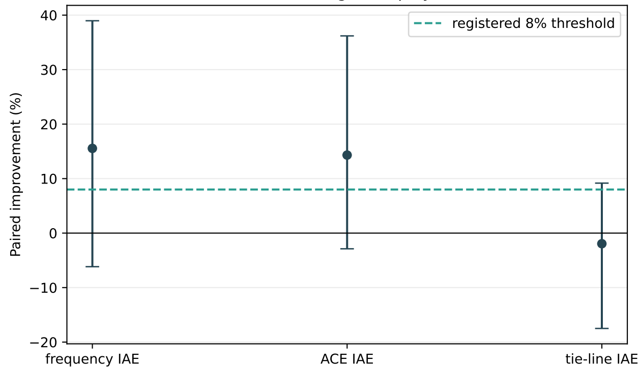
H7 DCSV-MPC vs strongest deployable baseline
