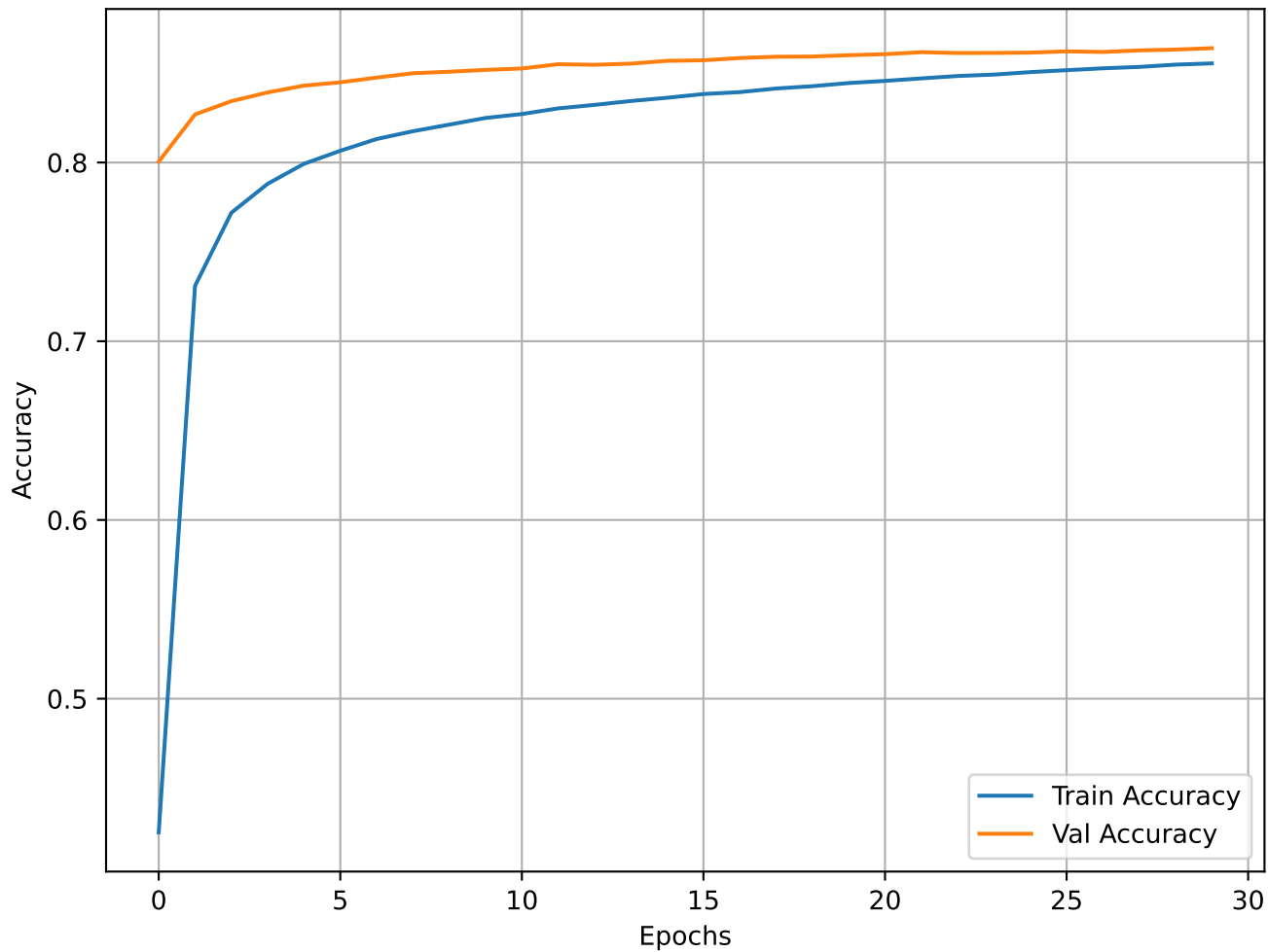
Accuracy Comparison
