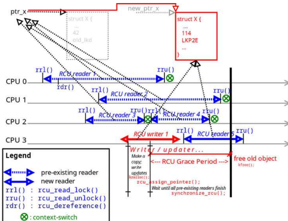
Figure 13.15: The same as Figure 13.14 ; plus the core RCU APIs are seen. After updating the data object, the writer waits for one RCU GP (up to the thick vertical line), and it then frees the old object; subsequent readers work upon the new data object
