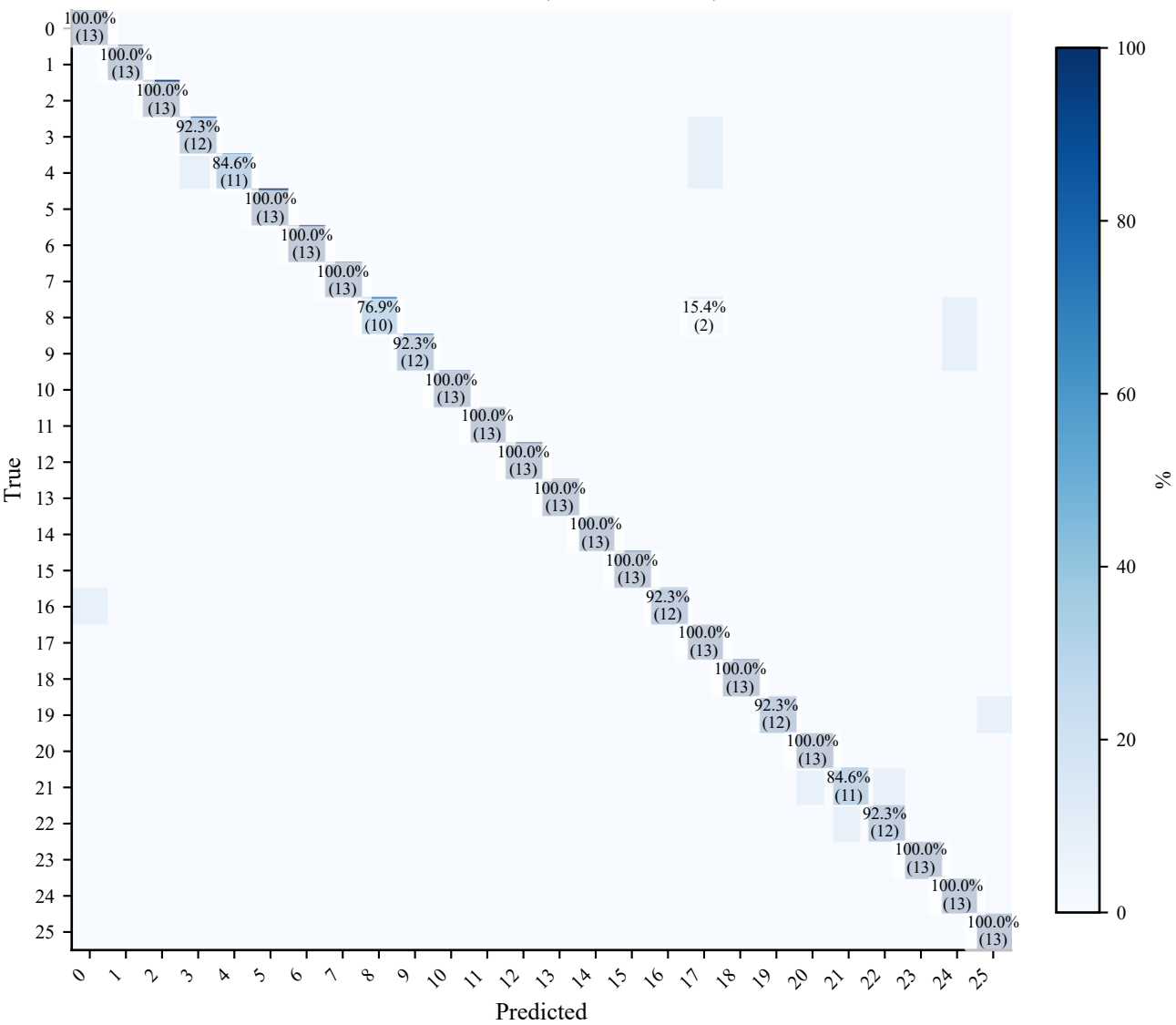
Confusion Matrix (Row-normalized)
