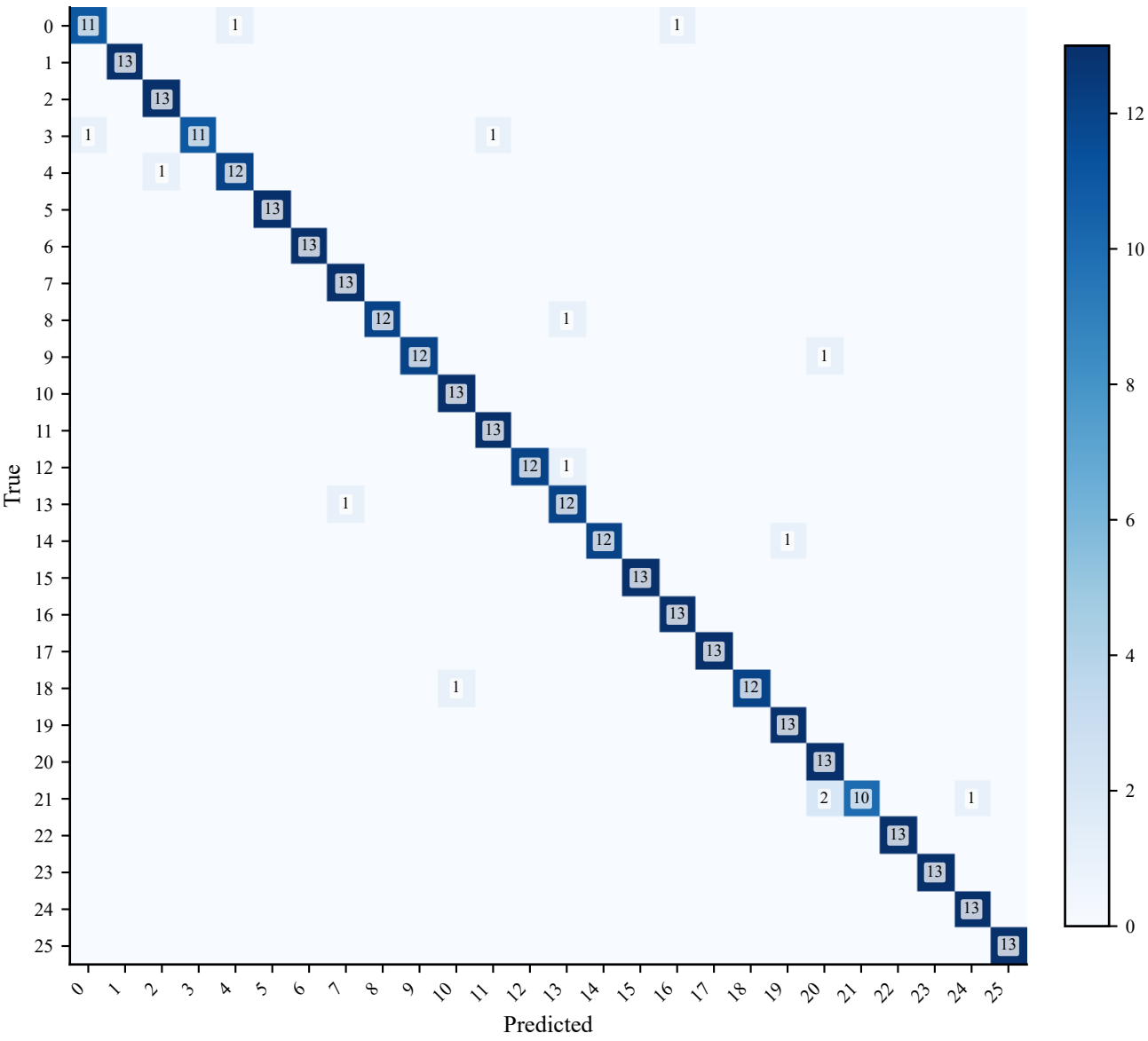
Confusion Matrix
