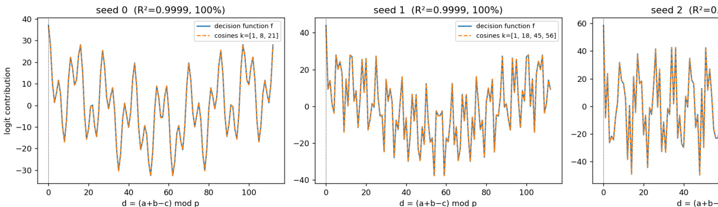
Figure 7: All three independently-trained seeds learn the same clock algorithm, each on its own set of key frequencies.
