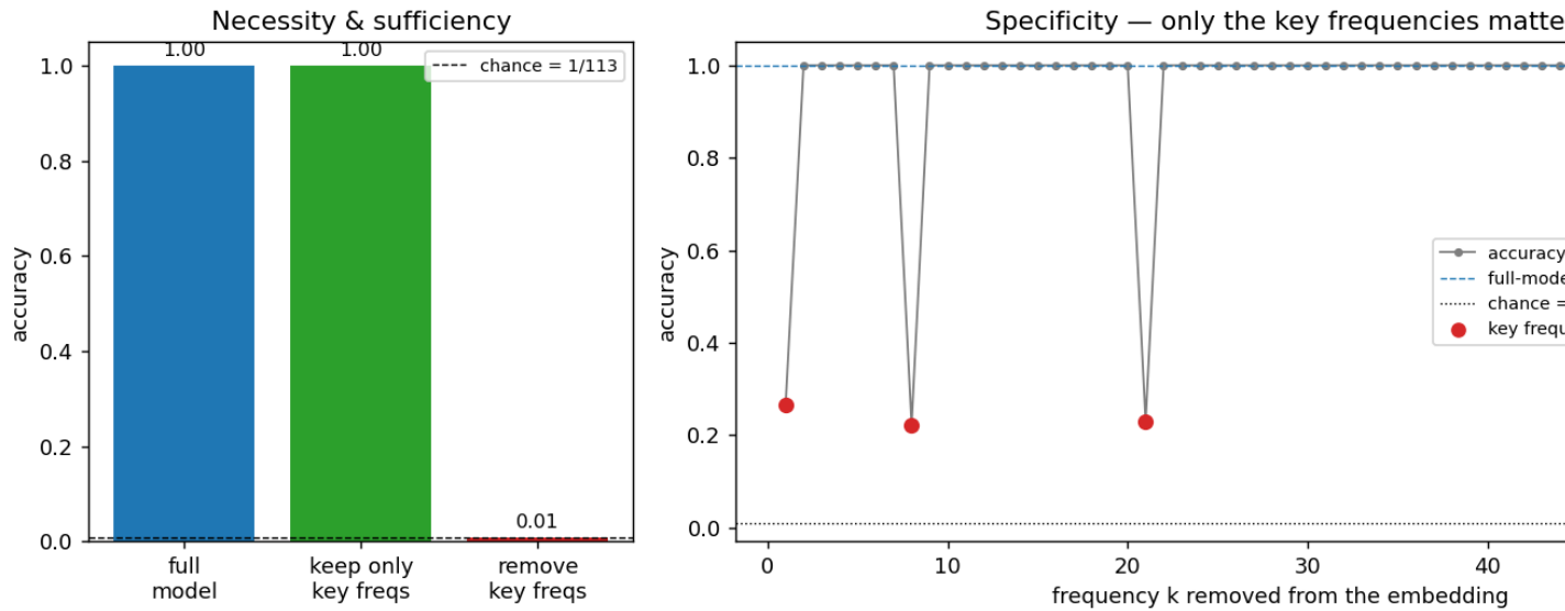
Figure 4: Keeping only the three key frequencies preserves 100% accuracy; removing them drops to chance; removing any other frequency does nothing.
