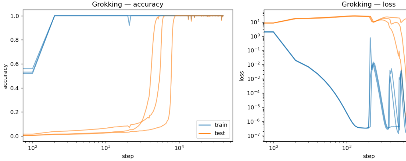
Figure 1: Across three seeds, training accuracy (blue) reaches 100% by step 200 while test accuracy (orange) stays at chance for thousands of steps before snapping to 100%.
