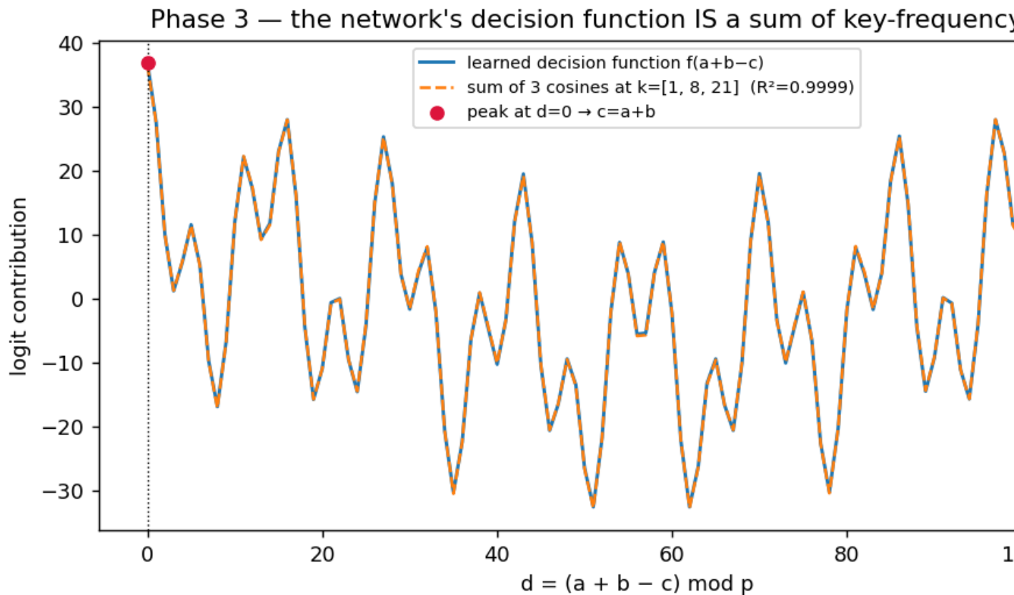
Figure 3: The learned decision function (blue) and a sum of three cosines (orange dashed) coincide at R^2 = 0.9999 , peaking at d = 0 ( c = a + b ).
