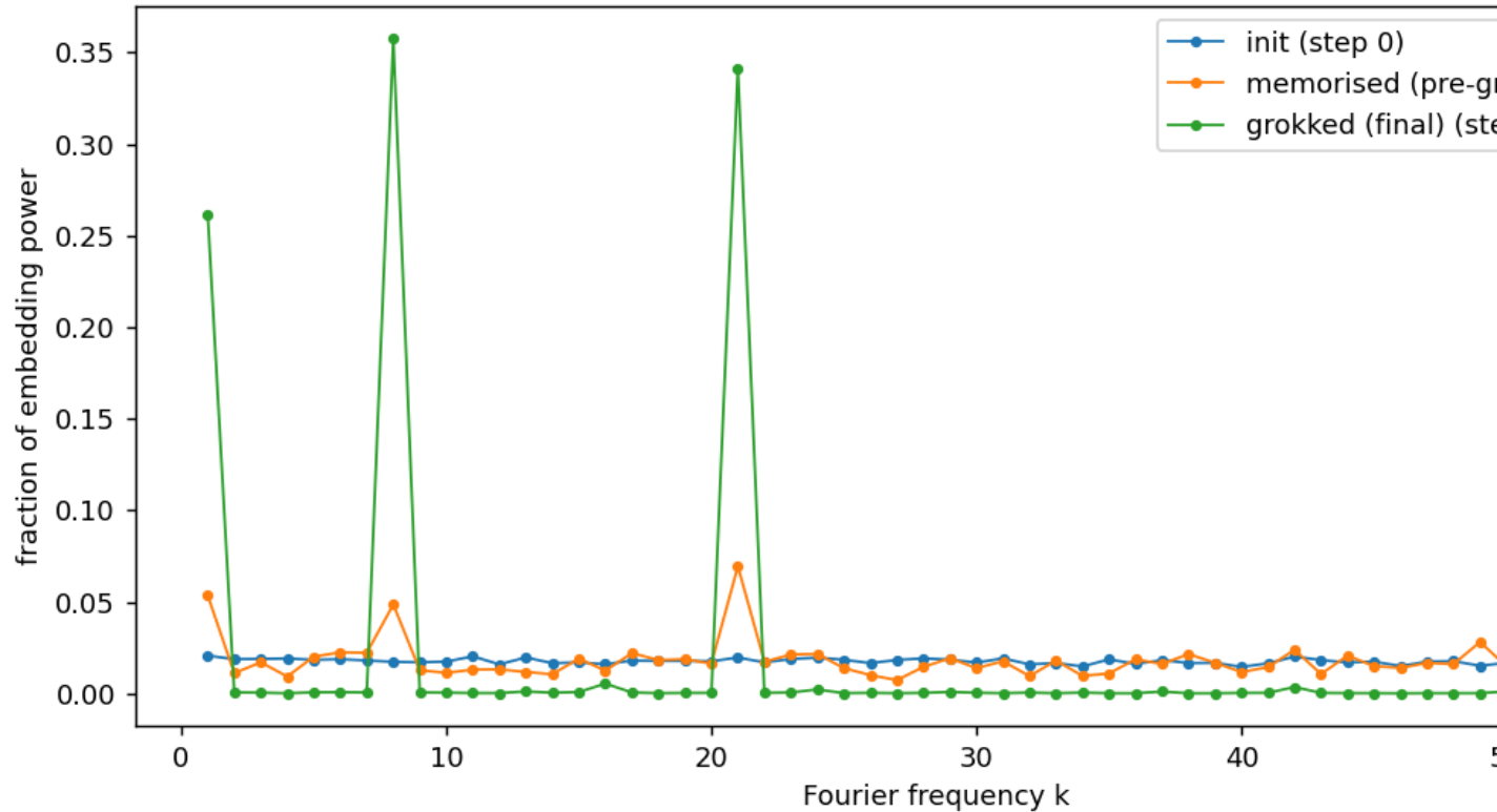
Figure 2: The grokked embedding (green) concentrates its power on three Fourier frequencies; the random-init (blue) and memorised-but-not-grokked (orange) embeddings are diffuse.
