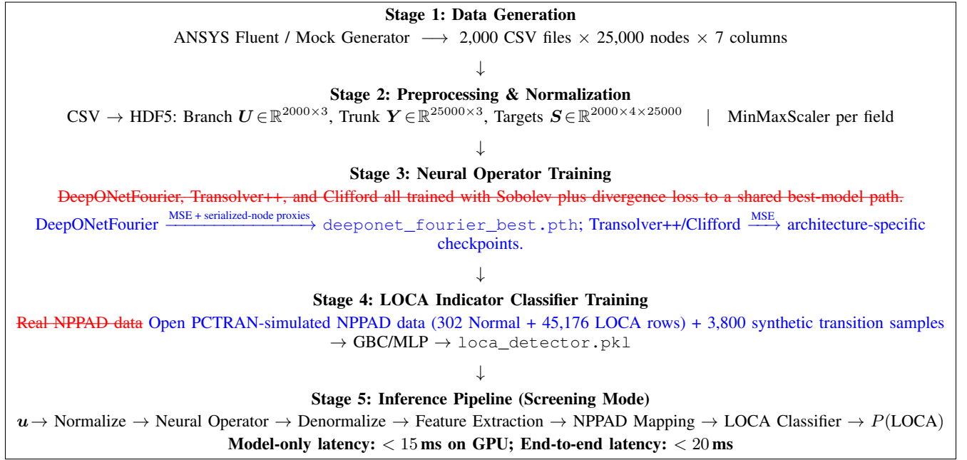
Fig. 1: End-to-end digital-twin proof-of-concept pipeline. Stages 1–4 run offline and Stage 5 executes the screening demonstration. The evaluated field data are synthetic, NPPAD records are PCTRAN-simulated, and this workflow is neither a plant protection system nor an operationally validated digital twin.
