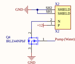
PUMP CONNECTORS
