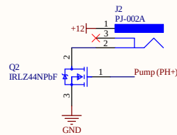
PUMP CONNECTORS
