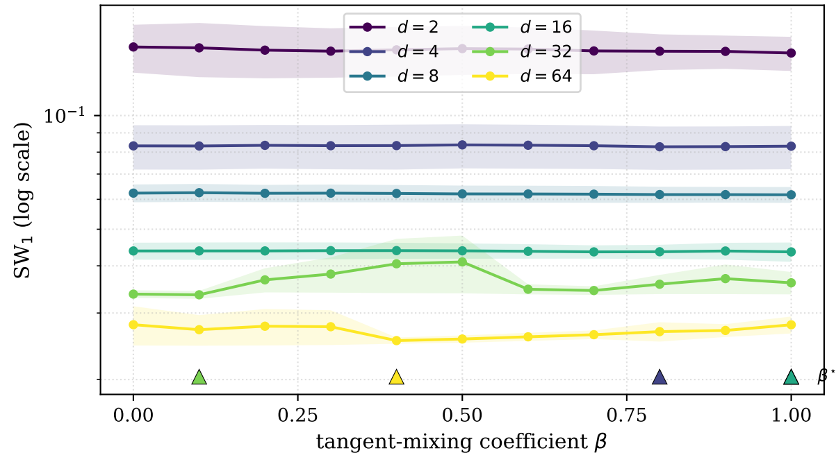
DGMM \beta -sweep across dimensions d \in \{2, 4, 8, 16, 32, 64\}
