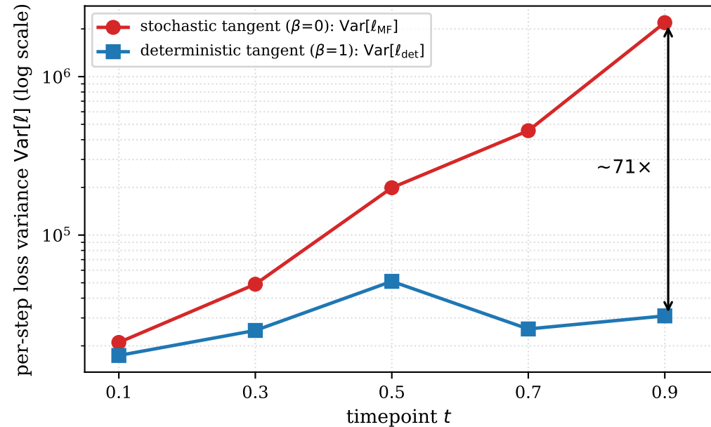
(a) J-amplification at DiT-B/4 scale (step 80k)
