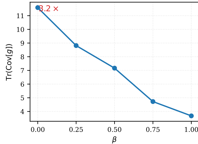
pinwheel
