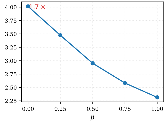
swiss_roll
