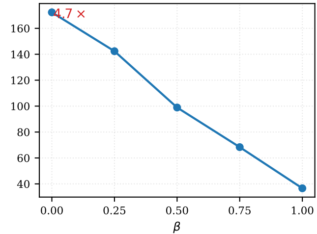
eight_gaussians
