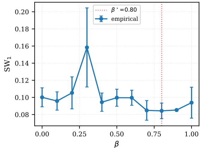
eight_gaussians
