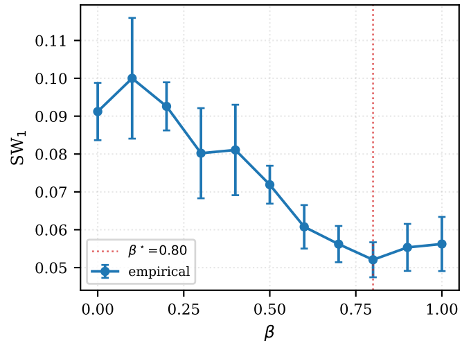
pinwheel
