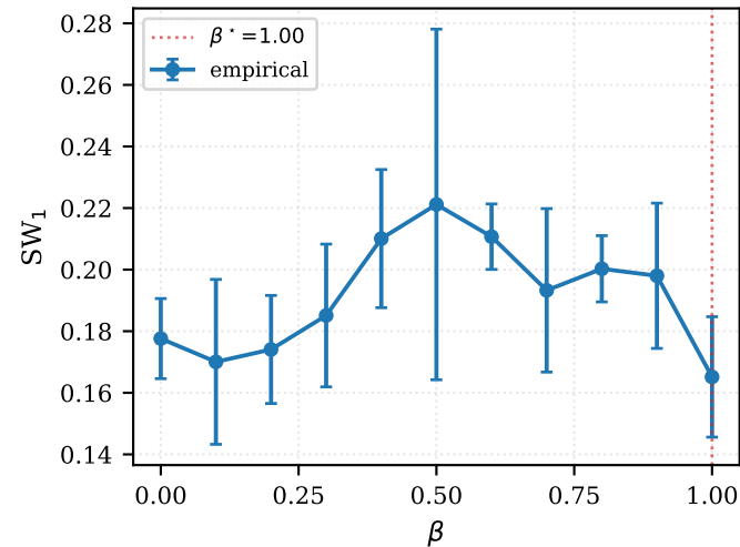
checkerboard
