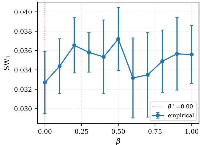
two_spirals
