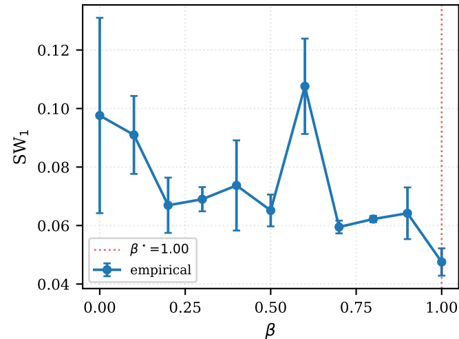
swiss_roll
