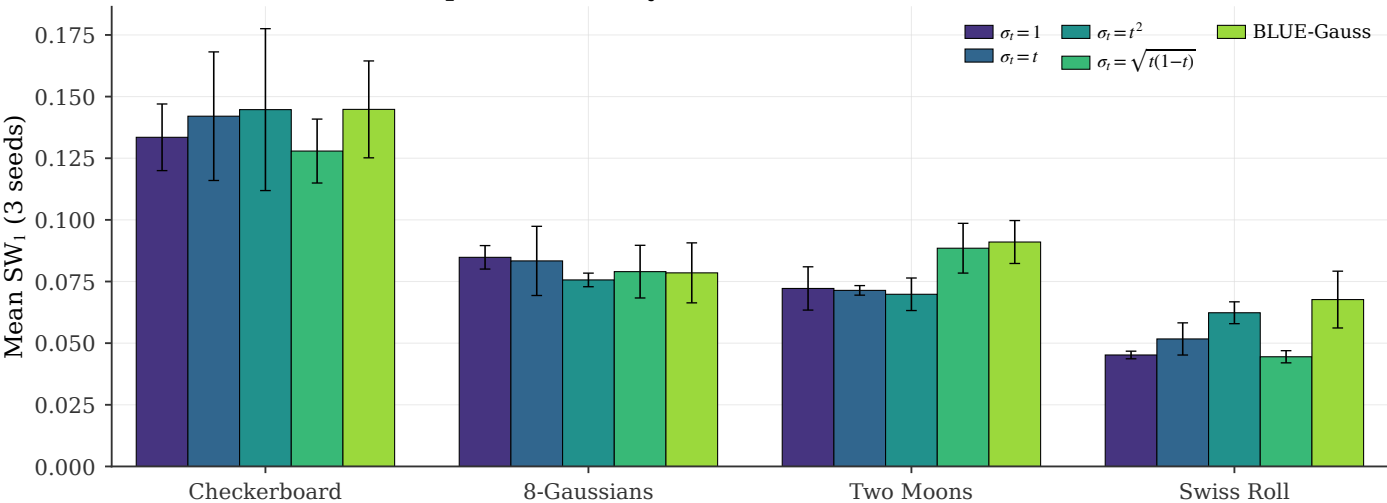
VaMF-TW: schedule sweep on the 2-D toy benchmark
