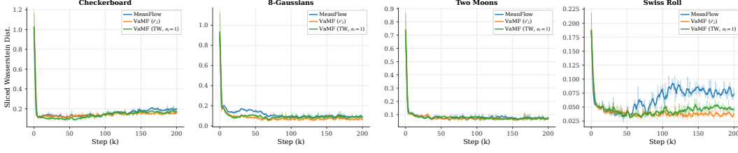
Figure 4: Convergence stability across the 2-D toy benchmark: SW_1 vs training step (smoothed) for each dataset. Vanilla MeanFlow plateaus with persistent high-frequency oscillations driven by the per-step gradient variance of theorem 1; VaMF- L_2 converges smoothly but to a higher floor than VaMF-TW with \sigma_t = 1 , and the gap between VaMF- L_2 and VaMF-TW is what the trace weight contributes.
