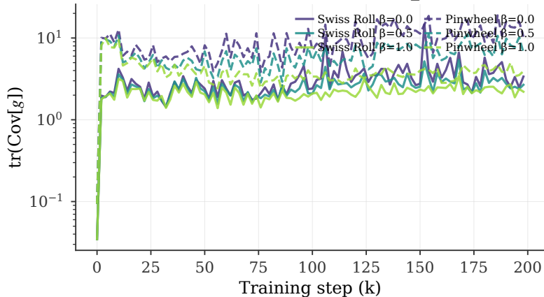
(b) Variance evolution (solid: swiss\_roll, dashed: pinwheel)
