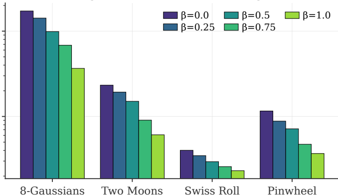
(a) Per-step gradient variance vs. tangent coefficient \beta
