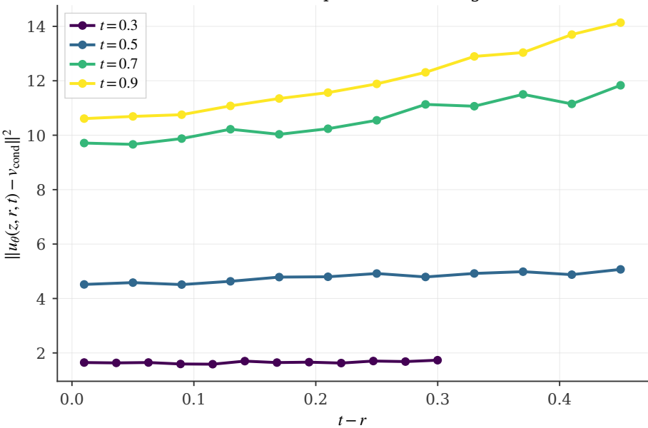
Curvature Gap vs Interval Length
