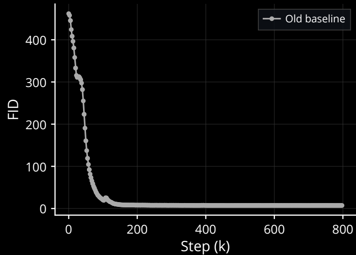
(c) FID Score
